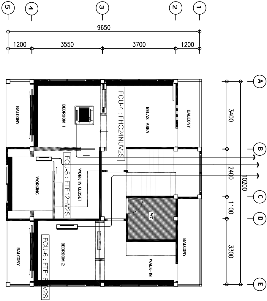
2 nd. AIRCONDITION & DUCT TYPE SYSTEM PLAN scale 1 : 1
